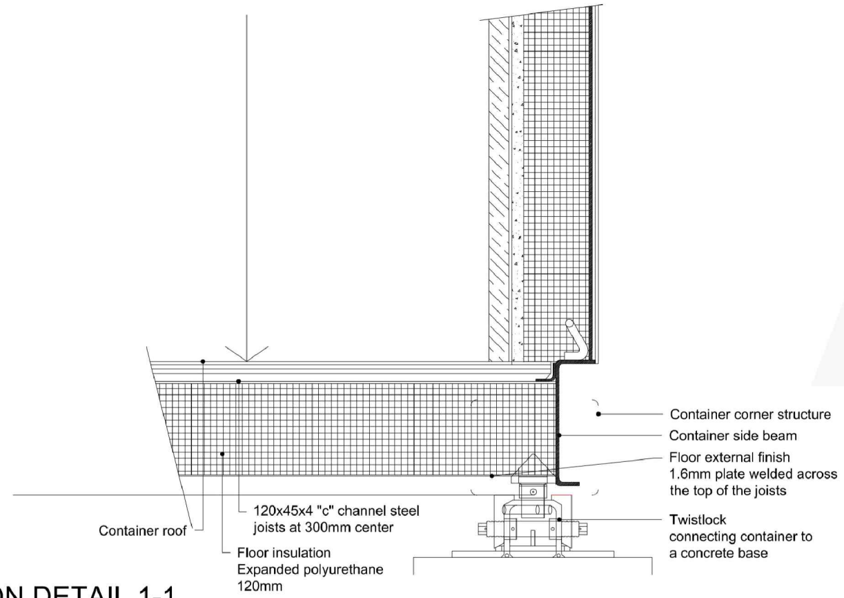
SECTION DETAIL 1-1
